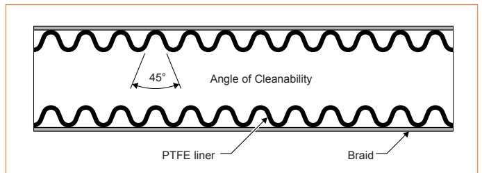
Typical Convoluted PTFE Hose
